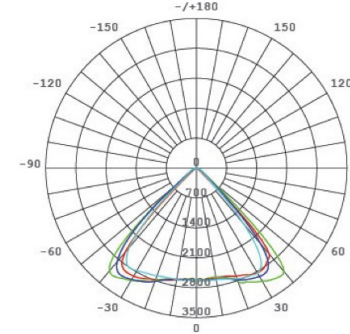
90°light distribution curve
