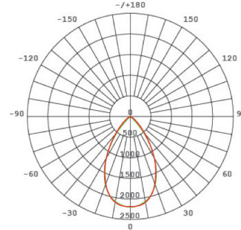
60°light distribution curve
