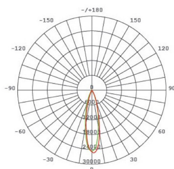
20°light distribution curve
