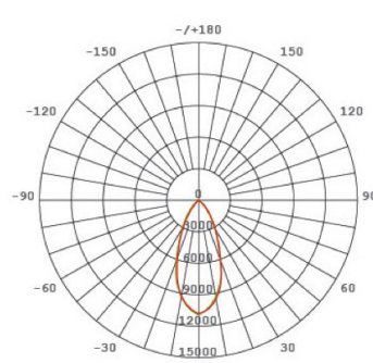
45°light distribution curve
